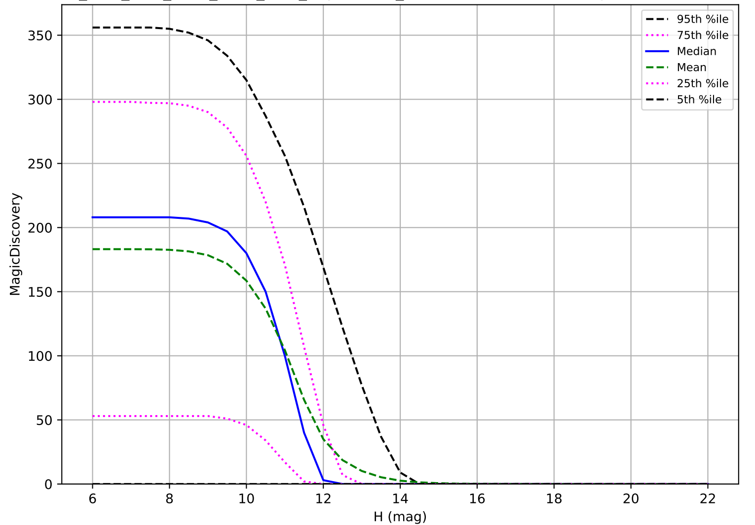
ddf_acor_sf15_lsf30_lsr10_v3.4_10yrs: OCC_r20 6 detections in 60 nights detection loss
