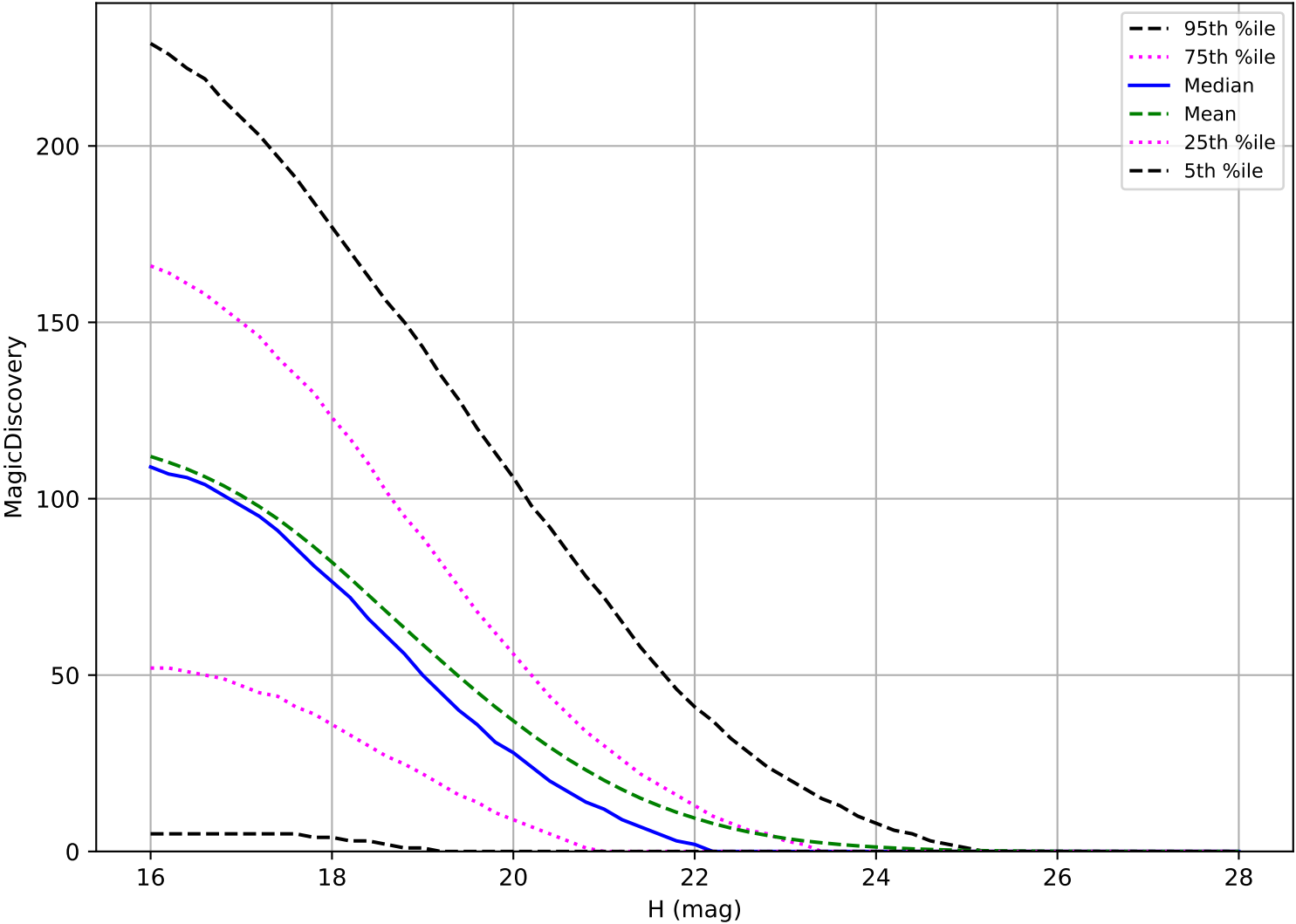
ddf_acor_sf15_lsf30_lsr10_v3.4_10yrs: NEO 6 detections in 60 nights detection loss
