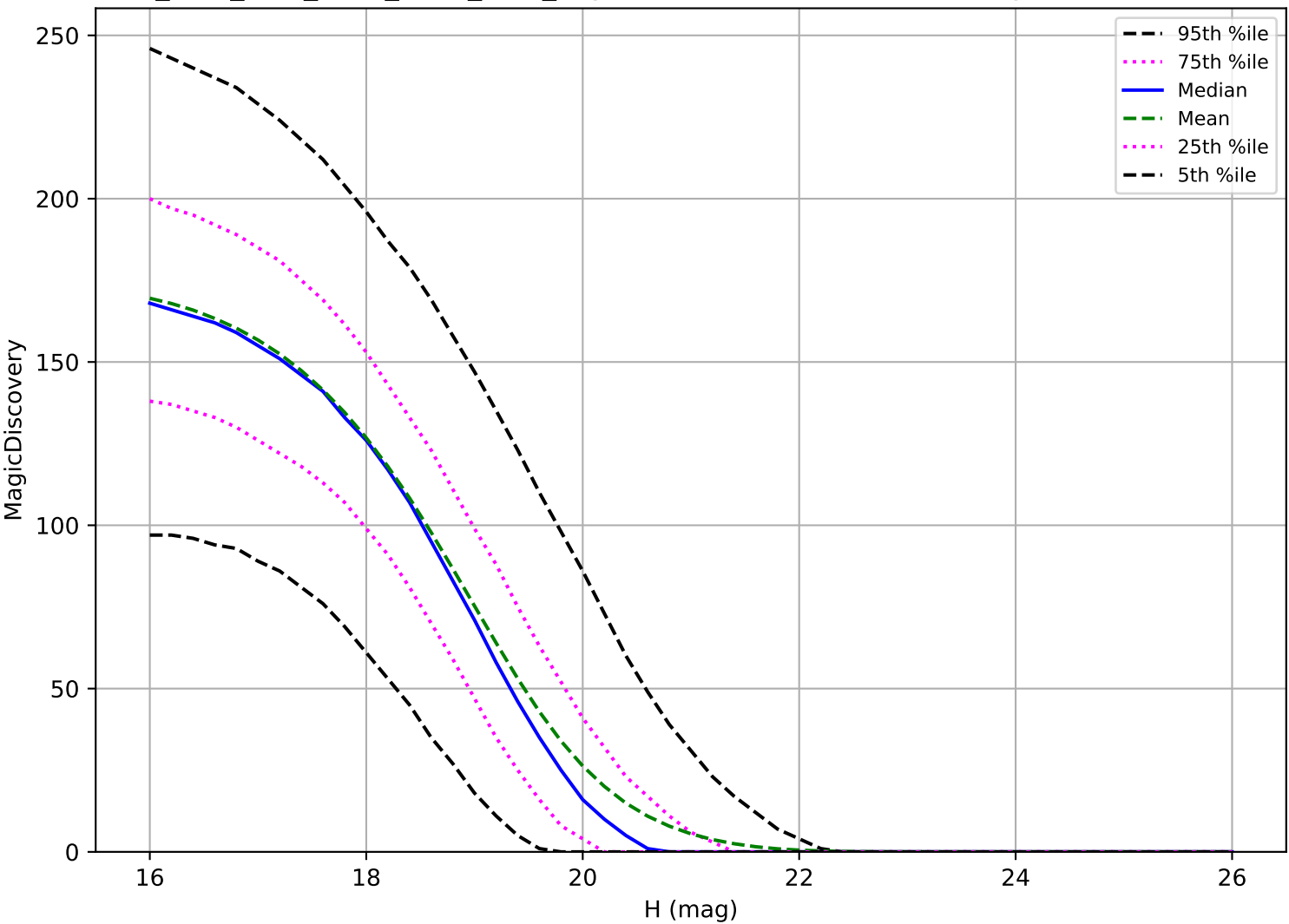
ddf_acor_sf15_lsf30_lsr10_v3.4_10yrs: MBA 6 detections in 60 nights detection loss
