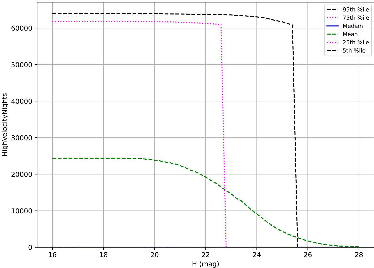
ddf_acor_sf15_lsf30_lsr10_v3.4_10yrs: PHA High velocity pair detection loss
