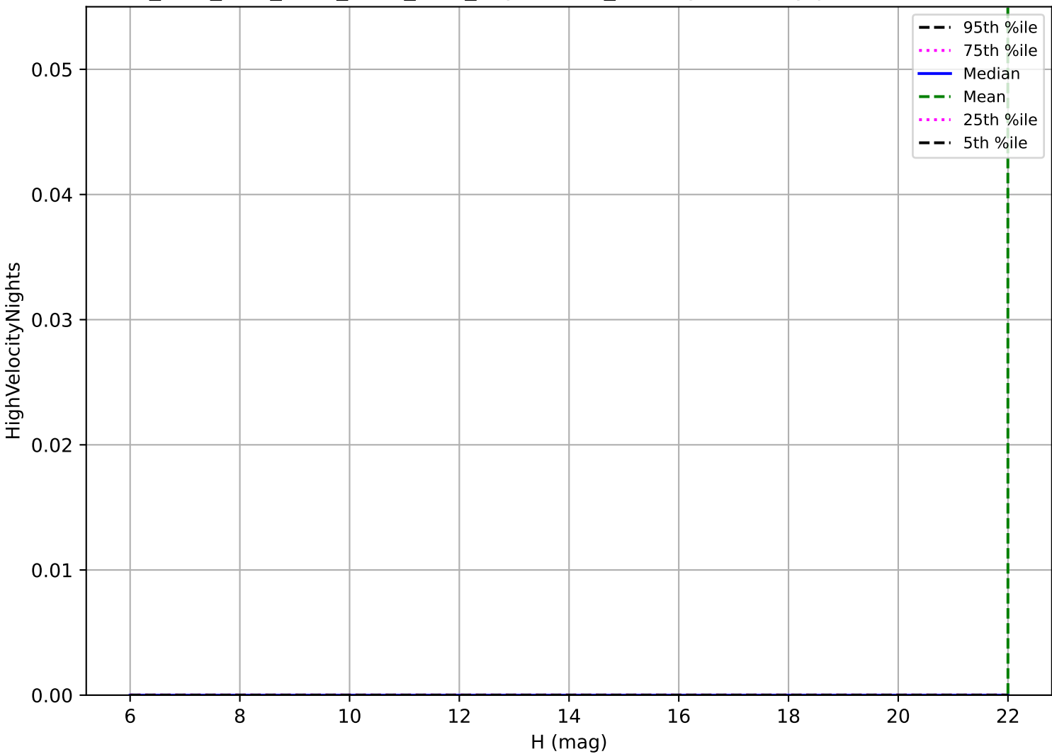
ddf_acor_sf15_lsf30_lsr10_v3.4_10yrs: OCC_r20 High velocity pair detection loss
