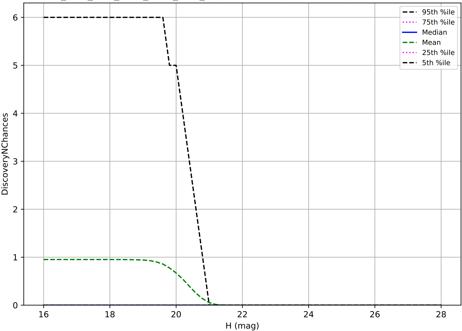
ddf_acor_sf15_lsf30_lsr10_v3.4_10yrs: Vatira 3 pairs in 15 nights detection loss
