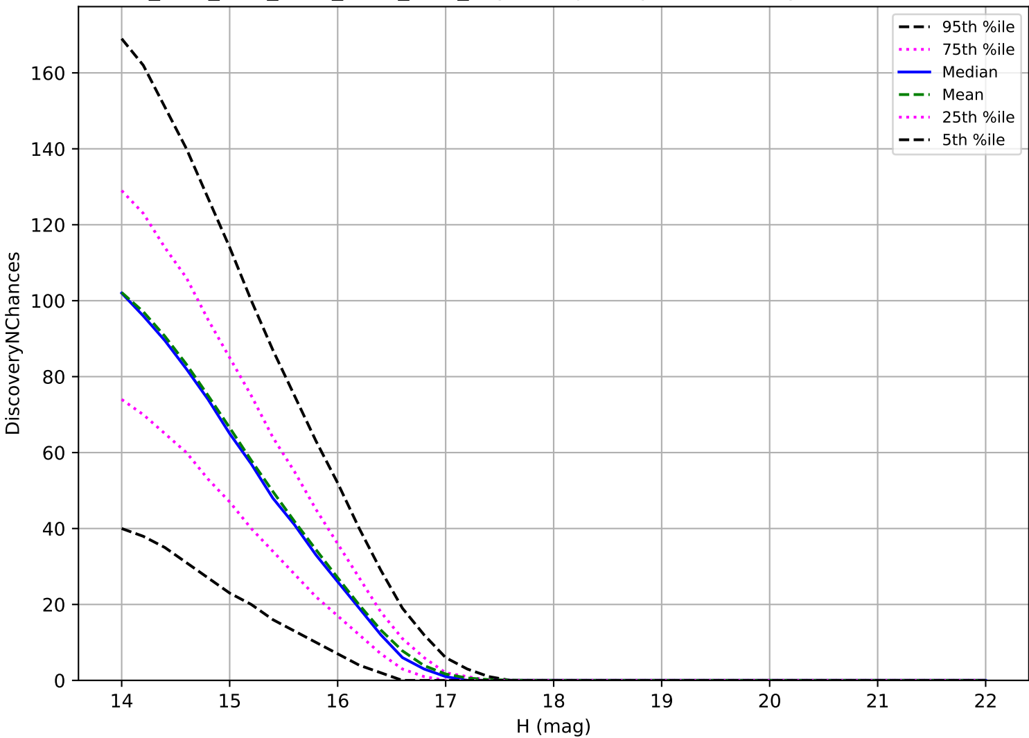
ddf_acor_sf15_lsf30_lsr10_v3.4_10yrs: Trojan 3 pairs in 15 nights detection loss
