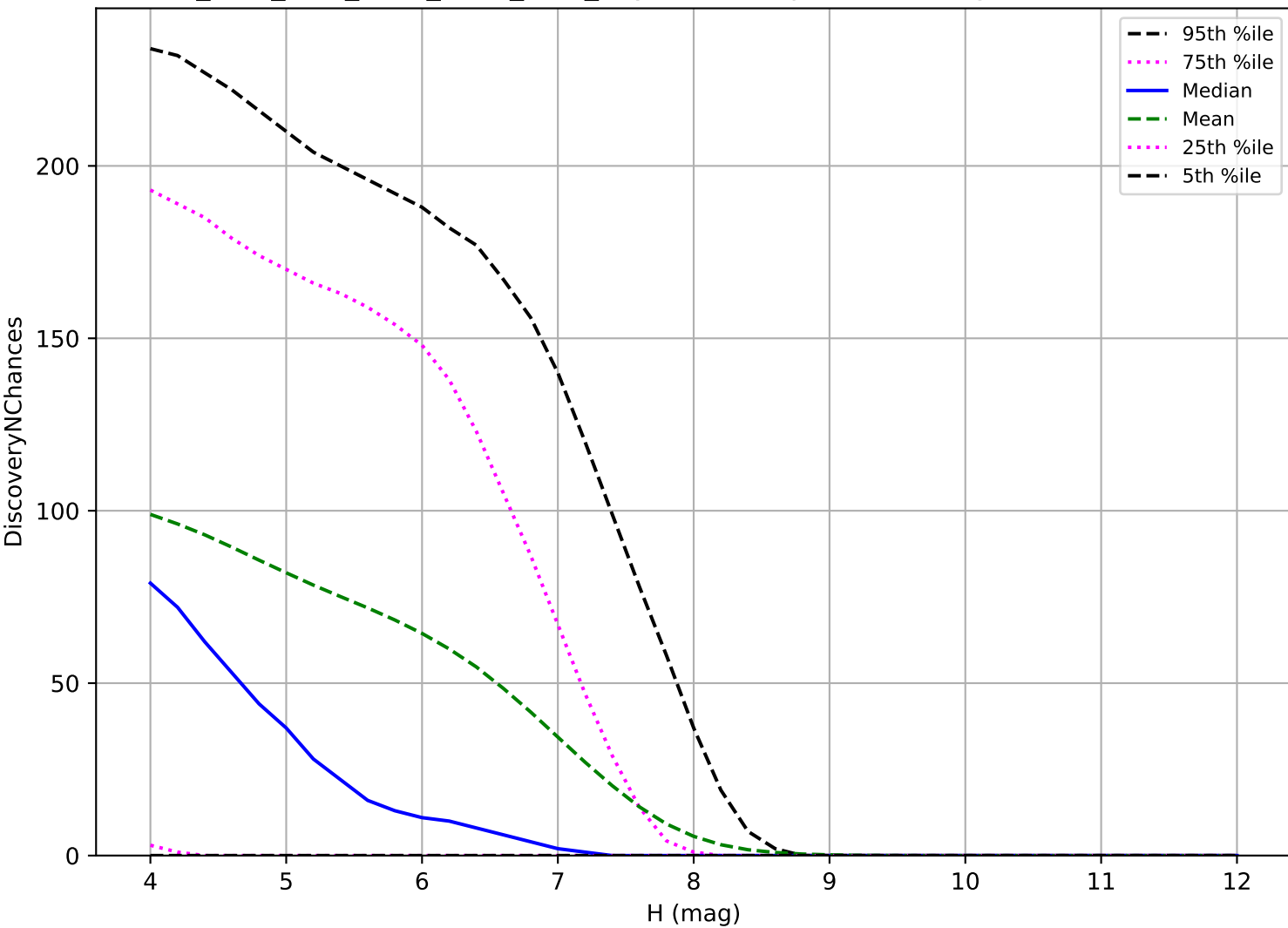
ddf_acor_sf15_lsf30_lsr10_v3.4_10yrs: TNO 3 pairs in 15 nights detection loss
