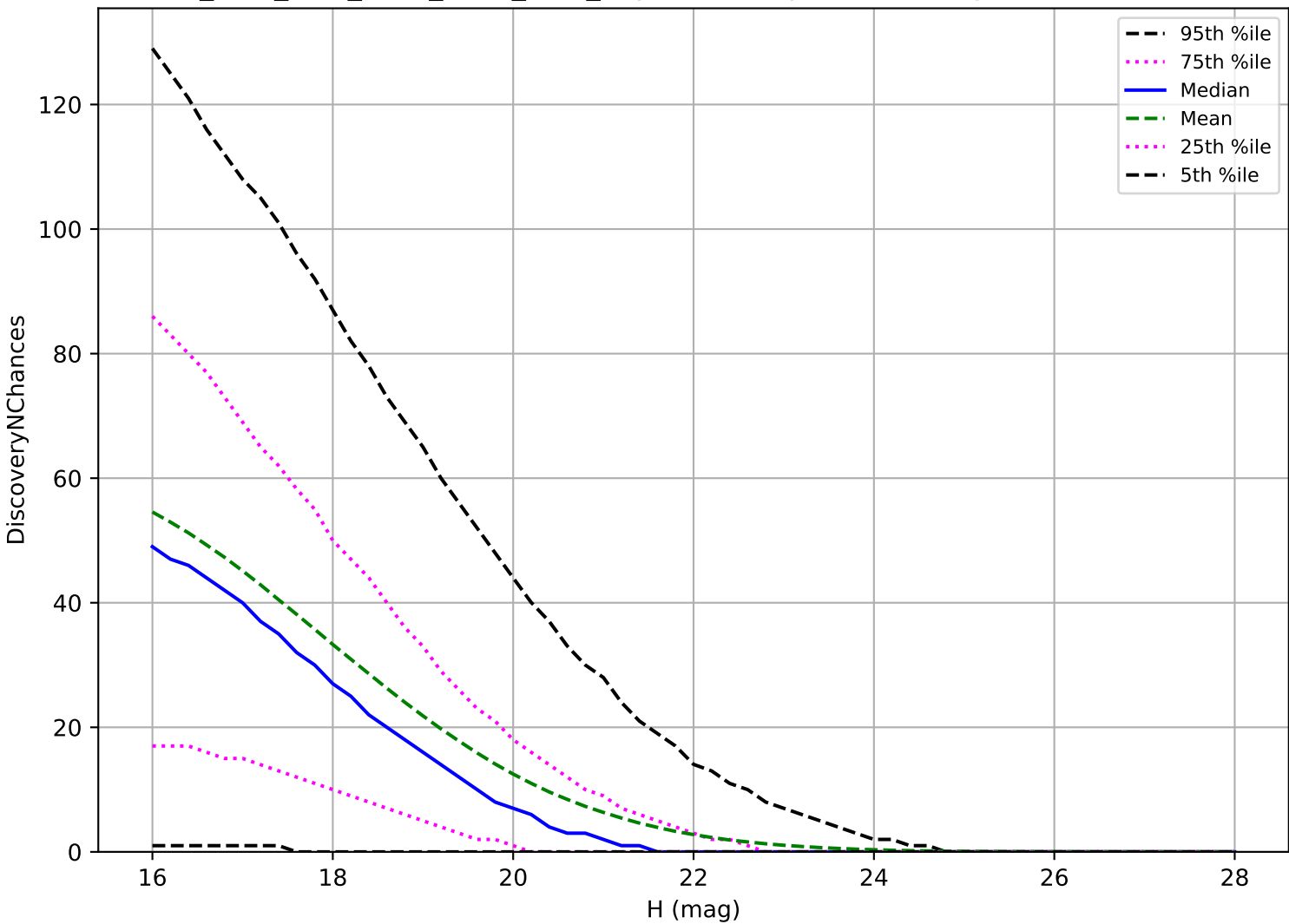
ddf_acor_sf15_lsf30_lsr10_v3.4_10yrs: PHA 3 pairs in 15 nights detection loss
