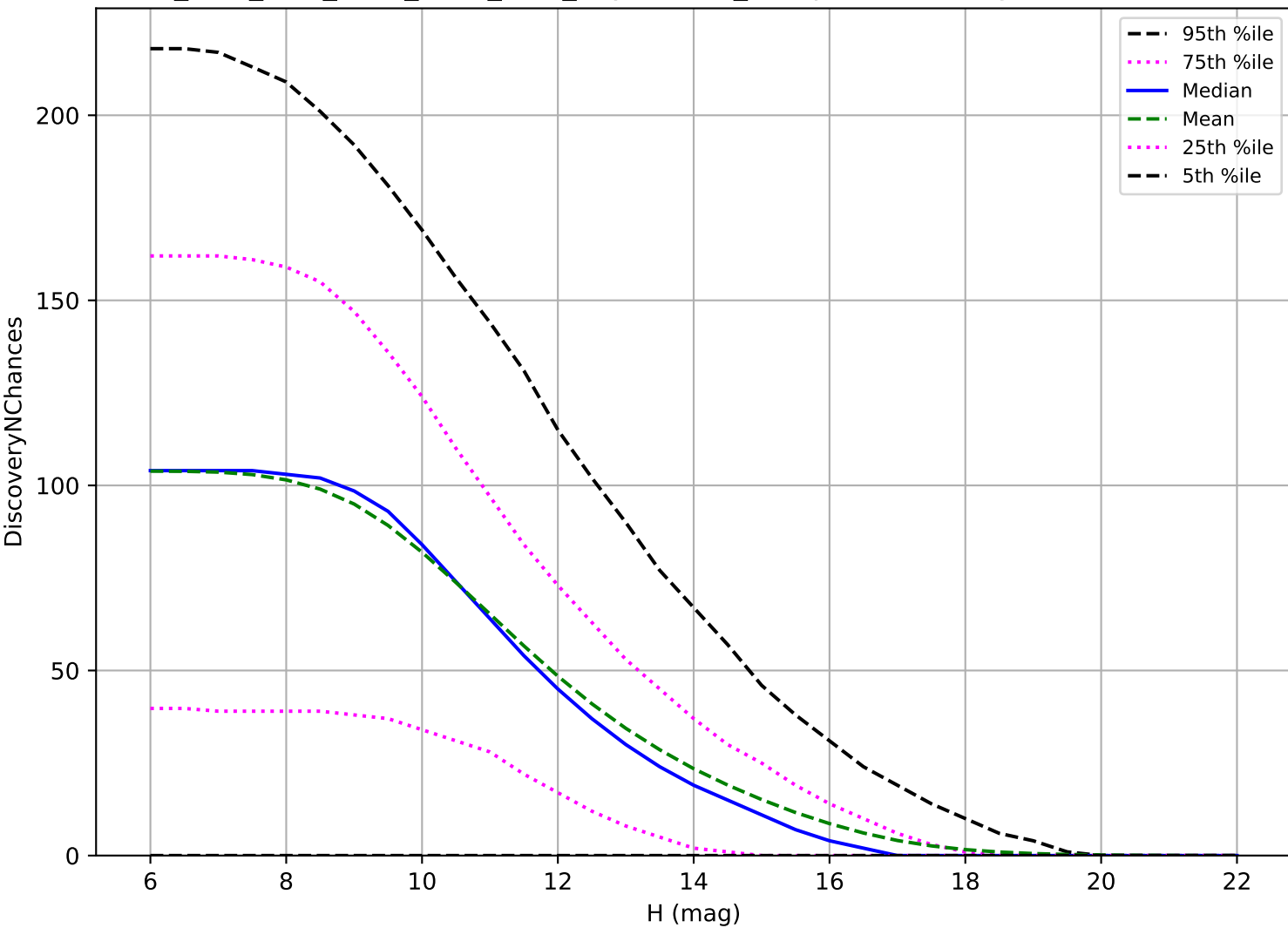
ddf_acor_sf15_lsf30_lsr10_v3.4_10yrs: OCC_r5 3 pairs in 15 nights detection loss
