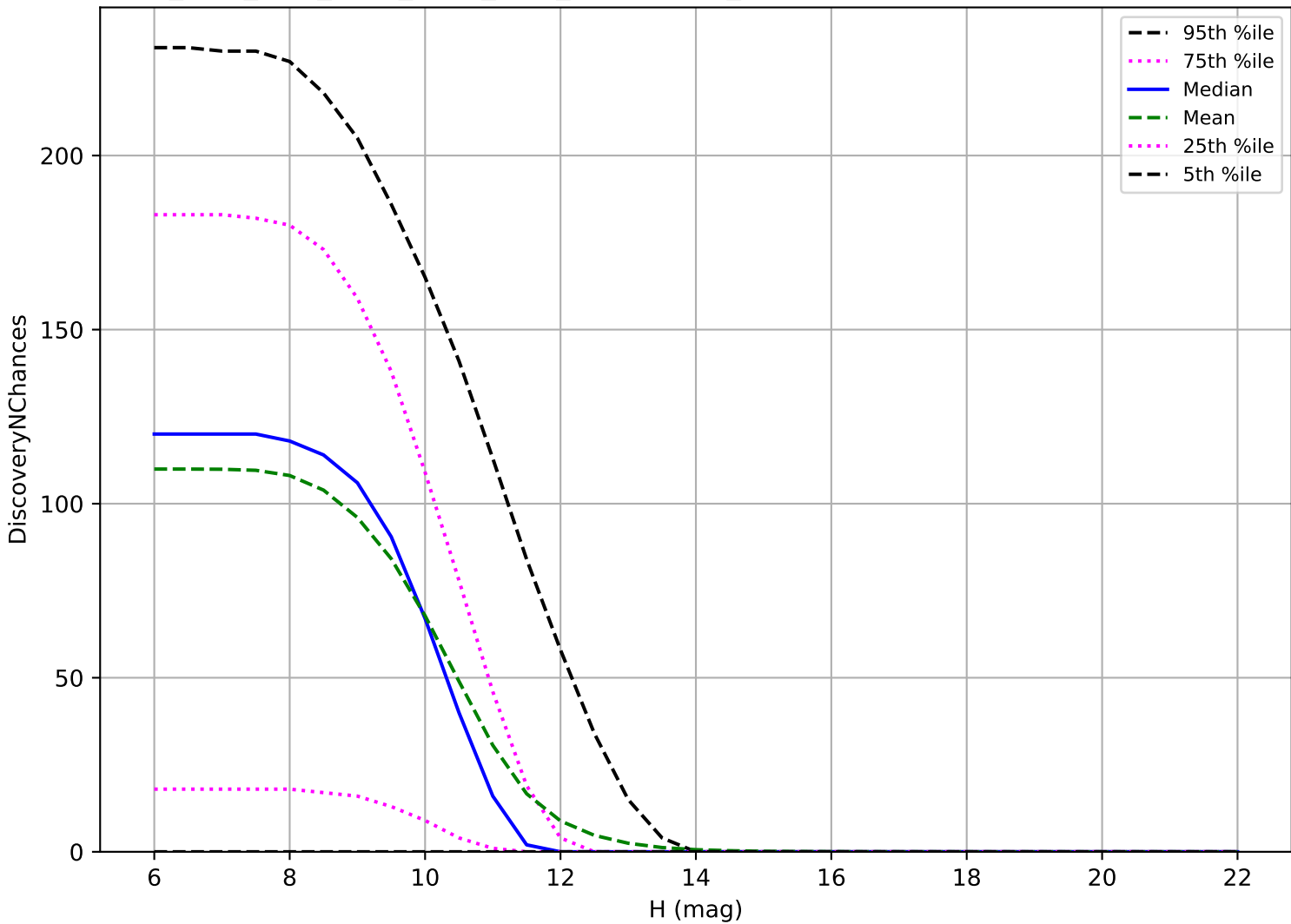
ddf_acor_sf15_lsf30_lsr10_v3.4_10yrs: OCC_r20 3 pairs in 15 nights detection loss
