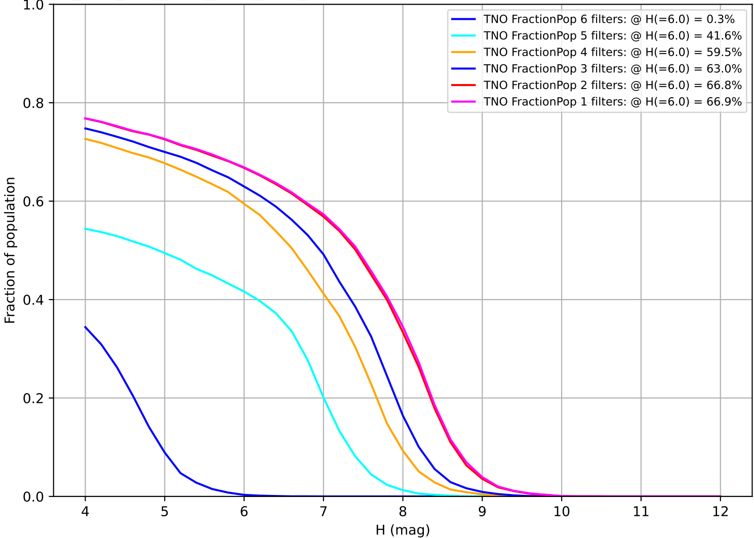
ddf_acor_sf15_lsf30_lsr10_v3.4_10yrs: Fraction of population with colors in X filters TNO
