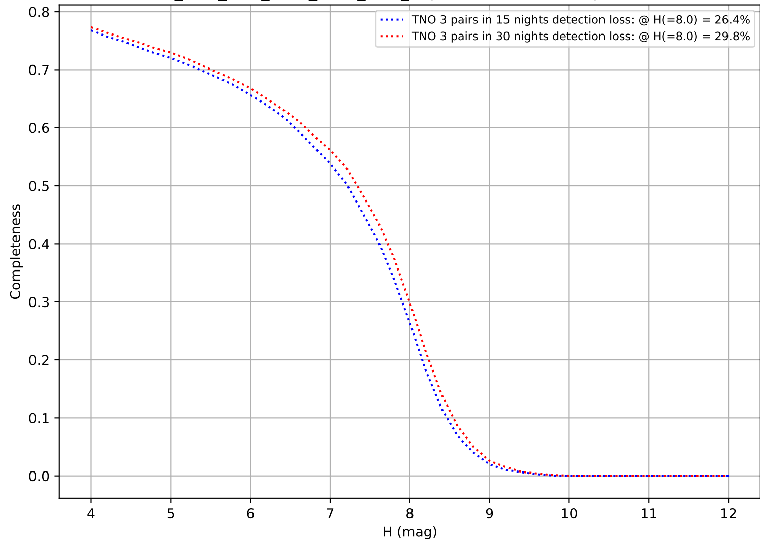
ddf_acor_sf15_lsf30_lsr10_v3.4_10yrs: DifferentialCompleteness
