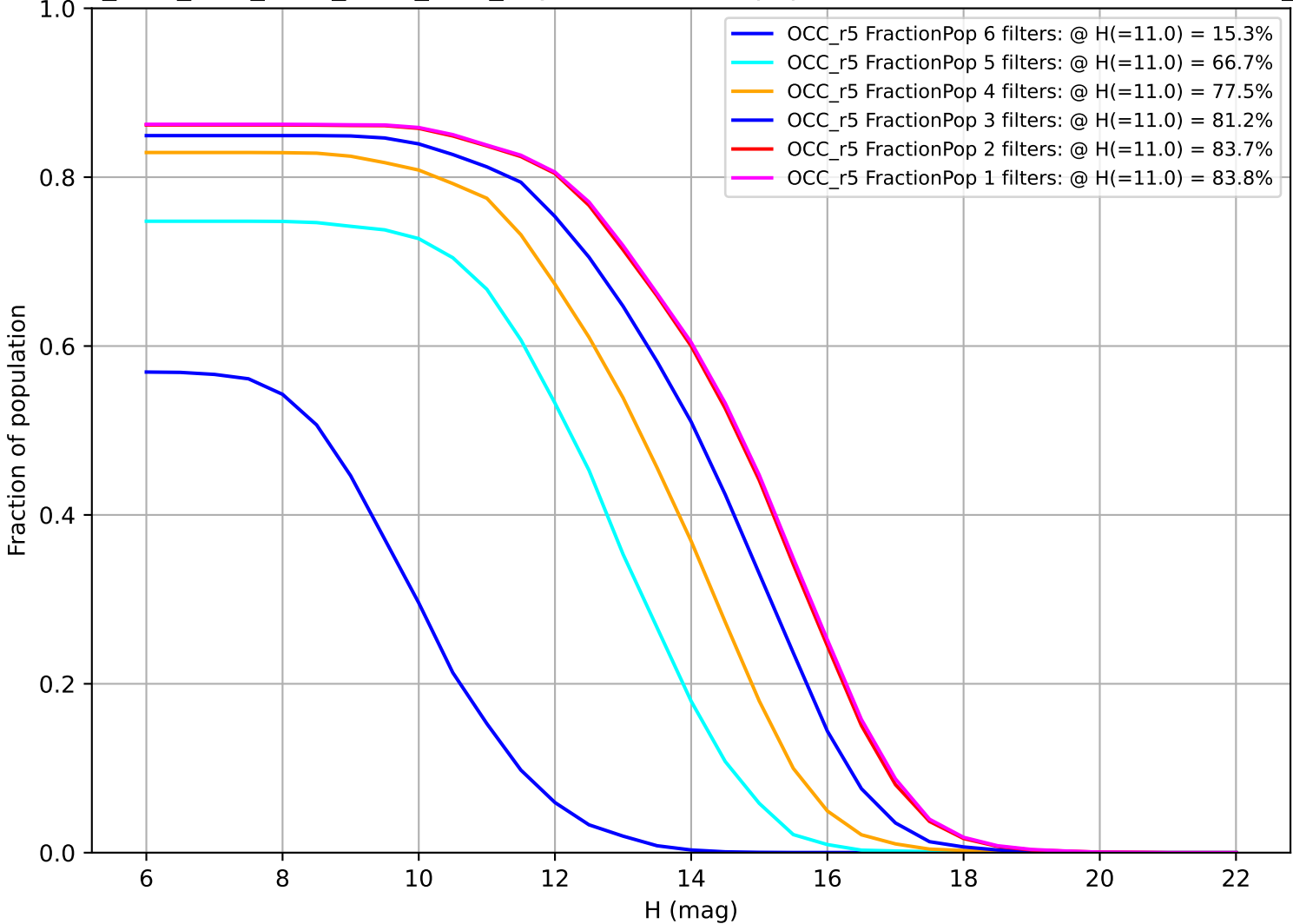
ddf_acor_sf15_lsf30_lsr10_v3.4_10yrs: Fraction of population with colors in X filters OCC_r5
