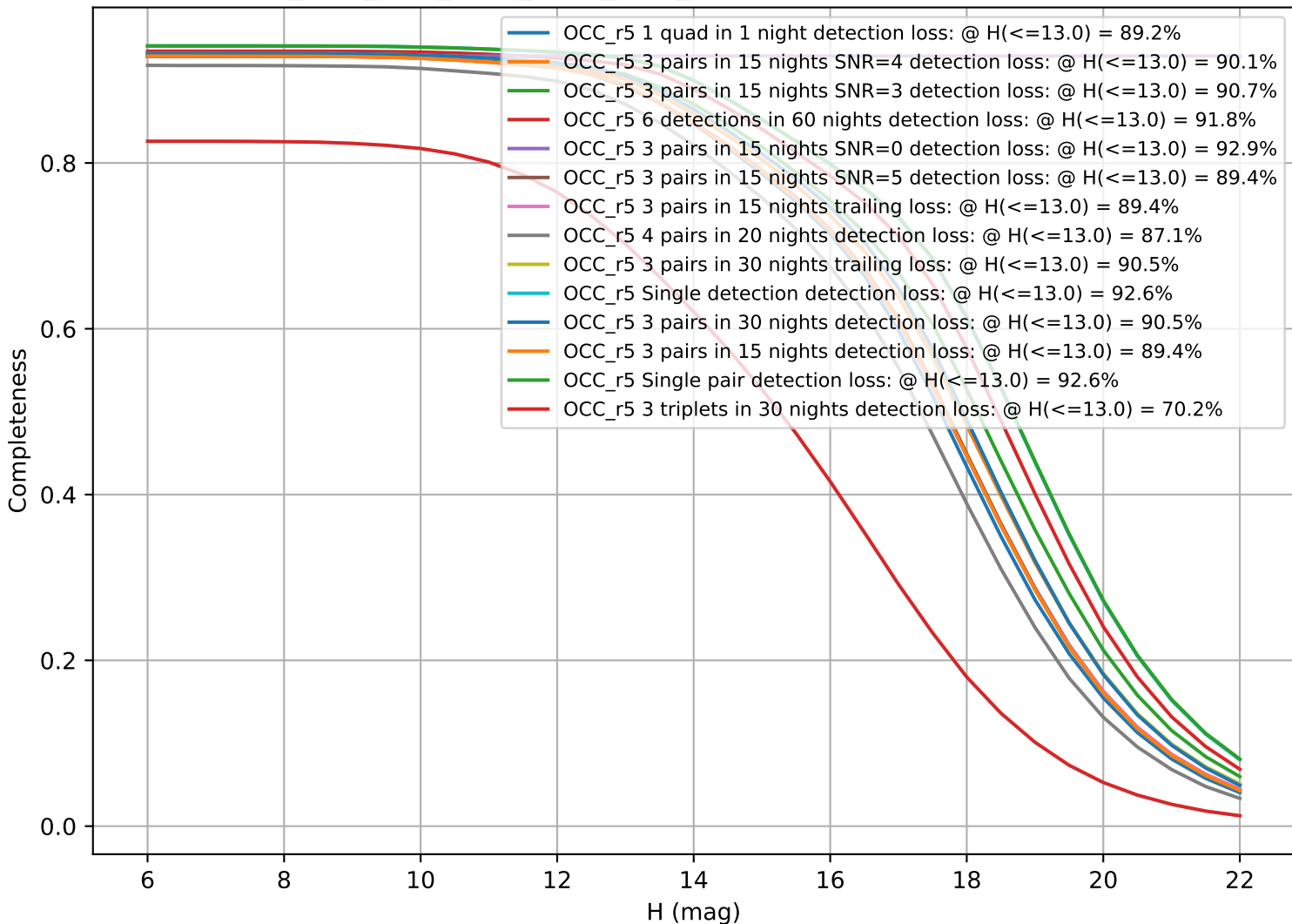
ddf_acor_sf15_lsf30_lsr10_v3.4_10yrs: CumulativeCompleteness
