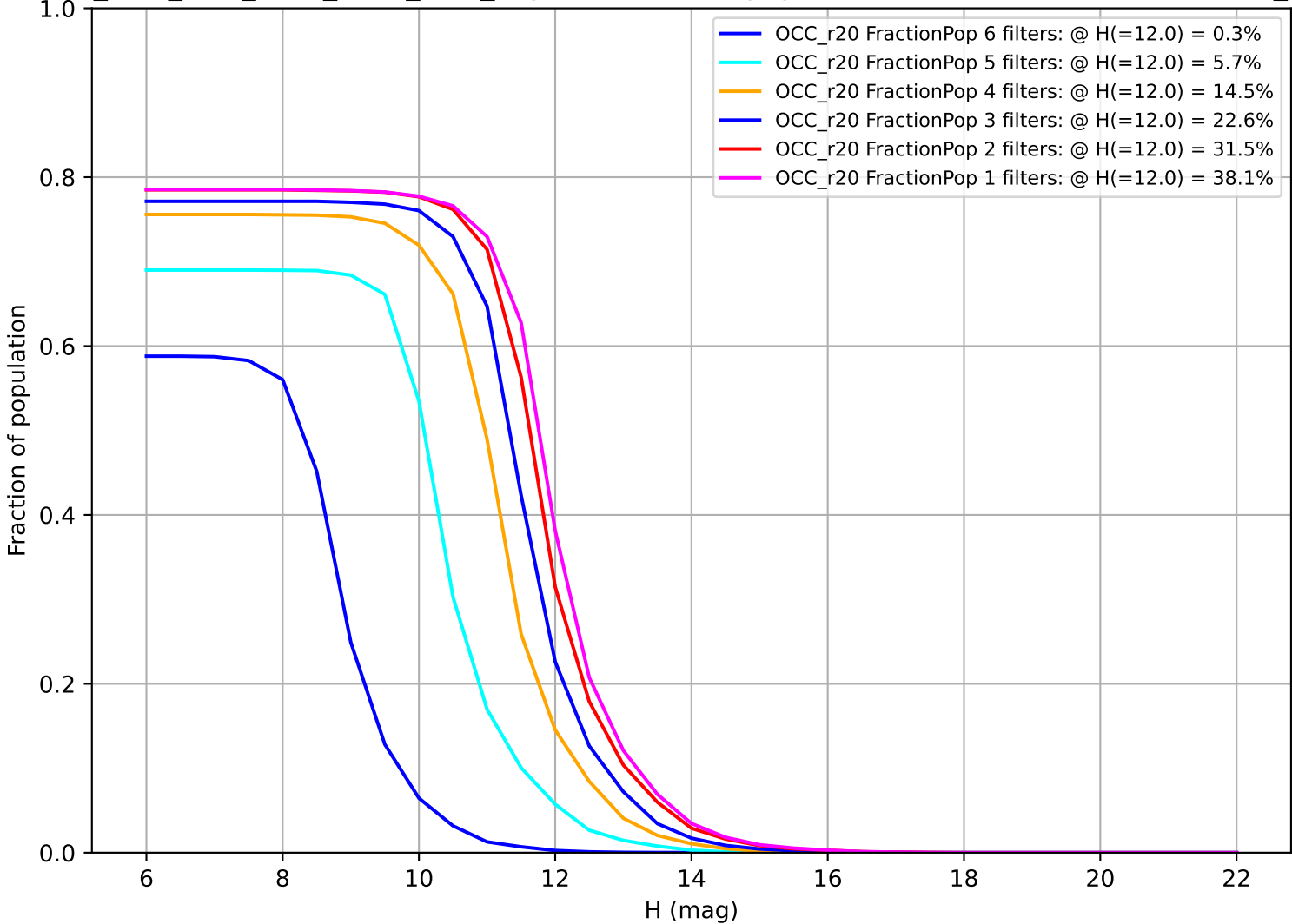
ddf_acor_sf15_lsf30_lsr10_v3.4_10yrs: Fraction of population with colors in X filters OCC_r20
