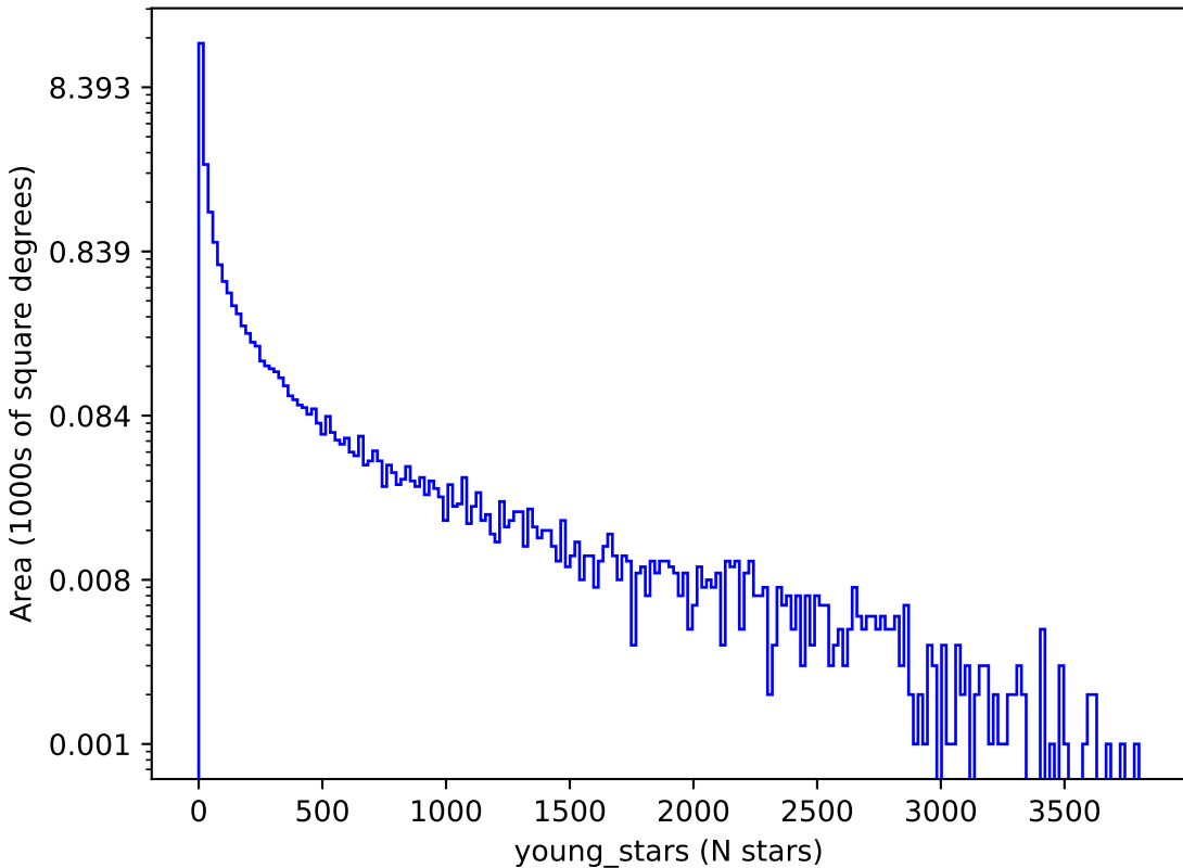
ddf_acor_sf15_lsf30_lsr10_v3.4_10yrs : young_stars
