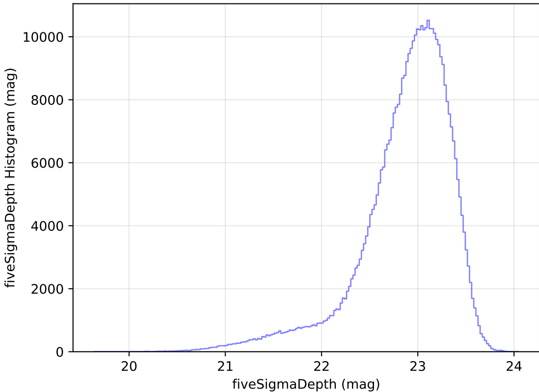
ddf_acor_sf15_lsf30_lsr10_v3.4_10yrs z: fiveSigmaDepth Histogram
