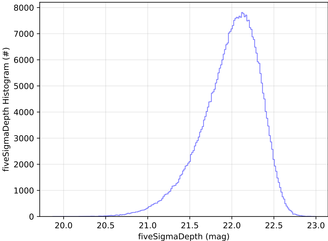
ddf_acor_sf15_lsf30_lsr10_v3.4_10yrs y: fiveSigmaDepth Histogram
