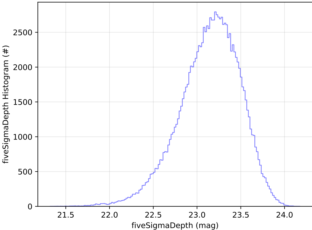
ddf_acor_sf15_lsf30_lsr10_v3.4_10yrs u: fiveSigmaDepth Histogram
