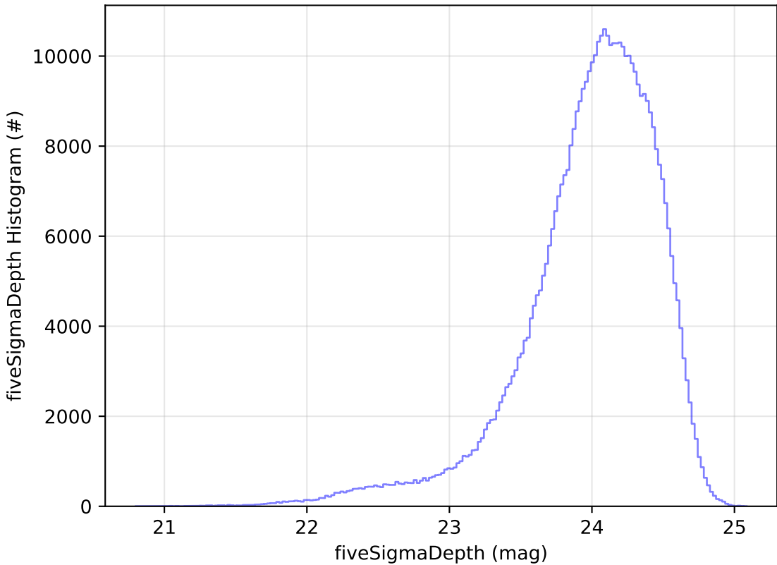
ddf_acor_sf15_lsf30_lsr10_v3.4_10yrs r: fiveSigmaDepth Histogram
