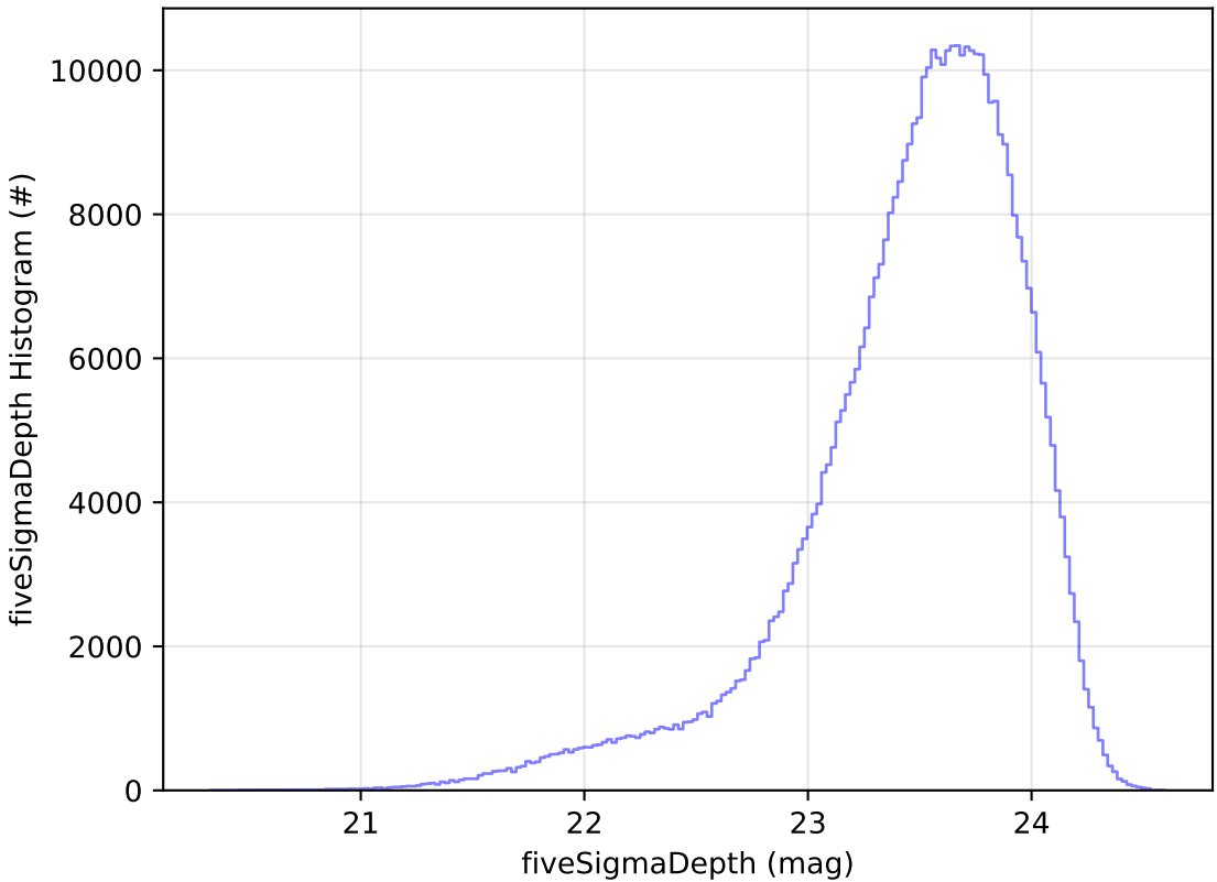
ddf_acor_sf15_lsf30_lsr10_v3.4_10yrs i: fiveSigmaDepth Histogram
