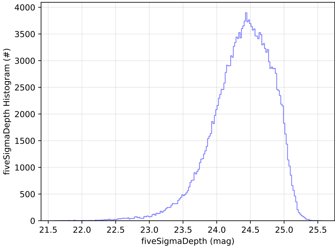
ddf_acor_sf15_lsf30_lsr10_v3.4_10yrs g: fiveSigmaDepth Histogram
