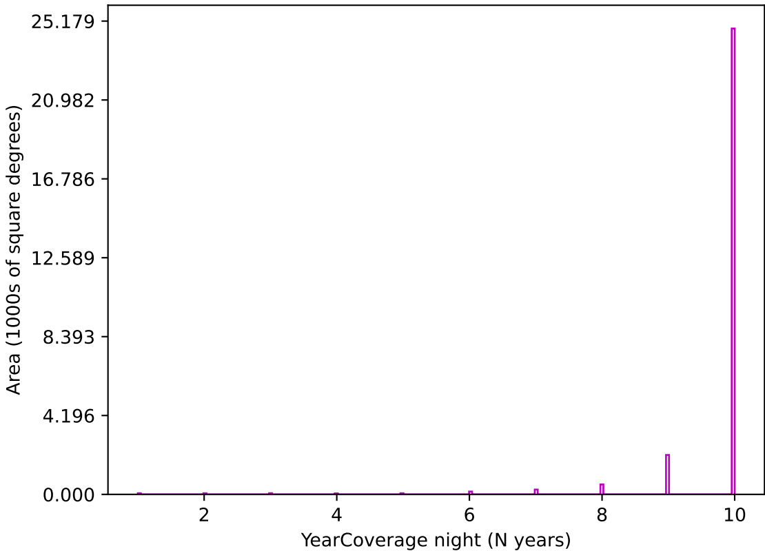
ddf_acor_sf15_lsf30_lsr10_v3.4_10yrs z band: YearCoverage night
