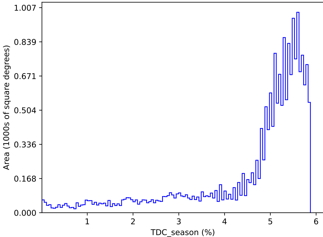
ddf_acor_sf15_lsf30_lsr10_v3.4_10yrs : TDC_season
