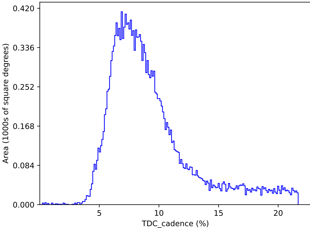
ddf_acor_sf15_ls30_lsr10_v3.4_10yrs : TDC_cadence
