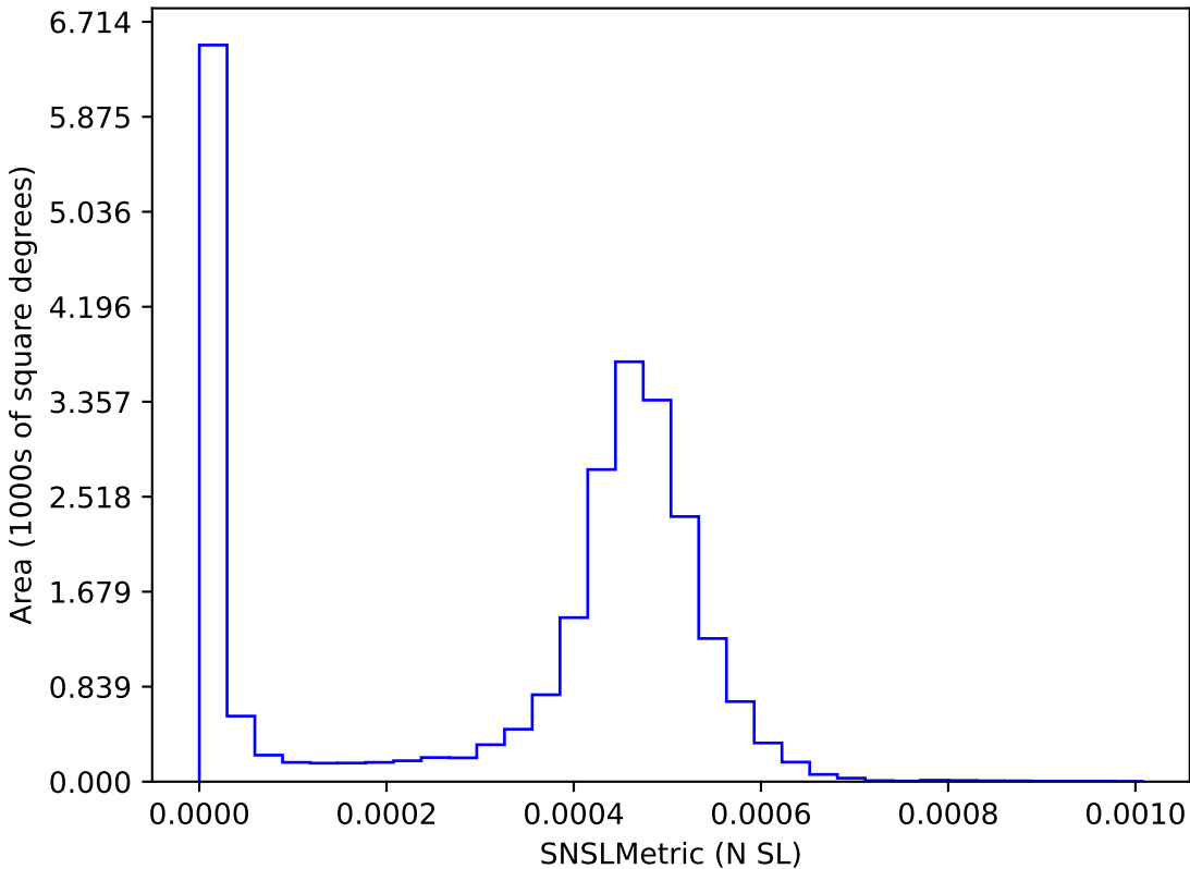
ddf_acor_sf15_lsf30_lsr10_v3.4_10yrs : SNSLMetric
