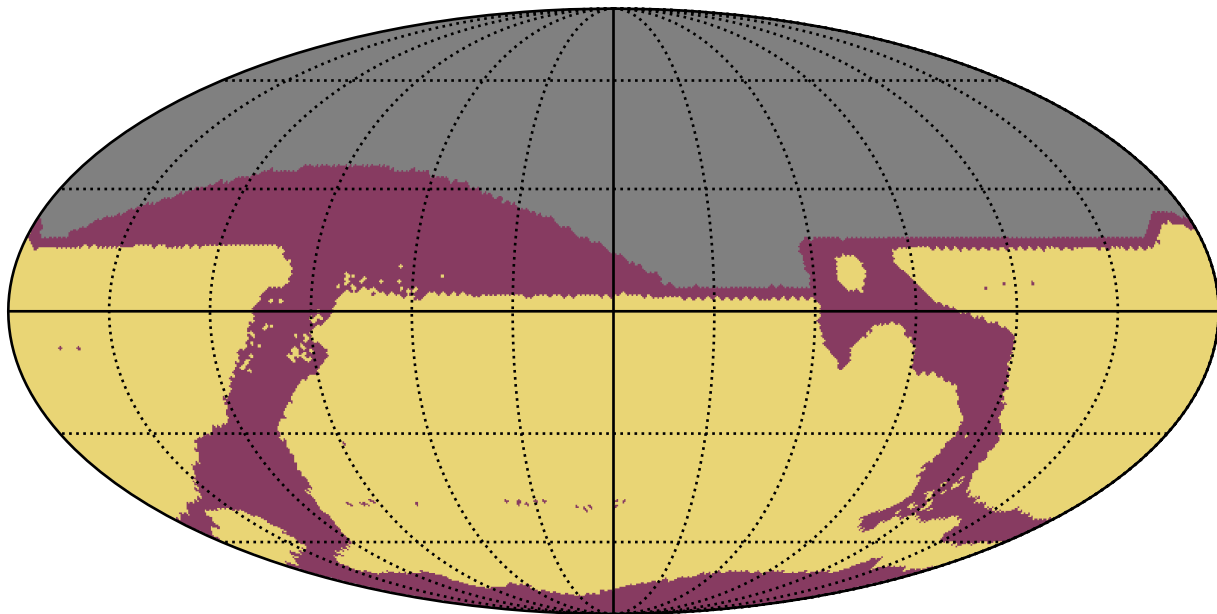
ddf_acor_sf15_lsf30_lsr10_v3.4_10yrs : RapidRevisits
