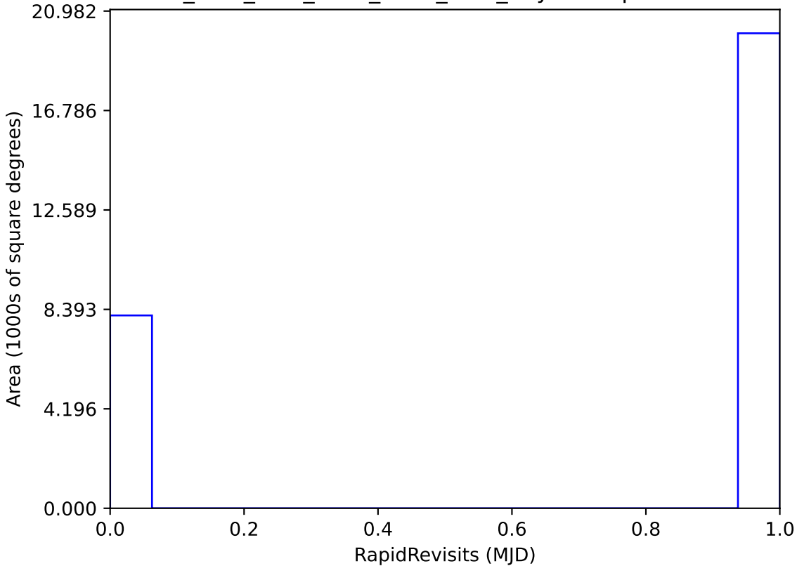
ddf_acor_sf15_lsf30_lsr10_v3.4_10yrs : RapidRevisits
