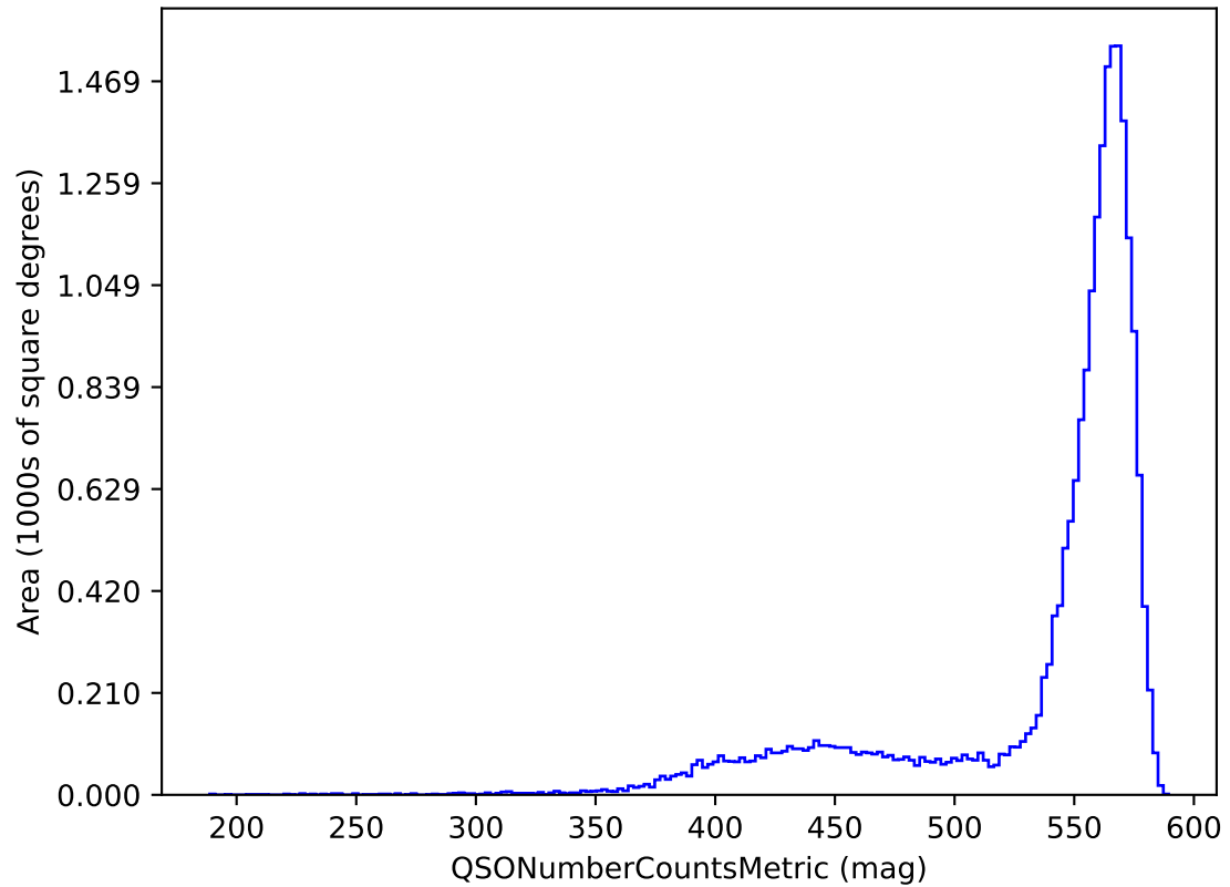
ddf_acor_sf15_lsf30_lsr10_v3.4_10yrs y band and non-DD: QSONumberCountsMetric
