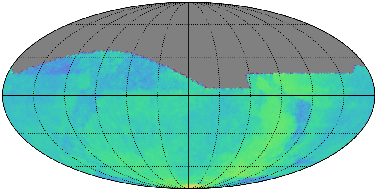
ddf_acor_sf15_lsf30_lsr10_v3.4_10yrs : Parallax Coverage @ 22.4
