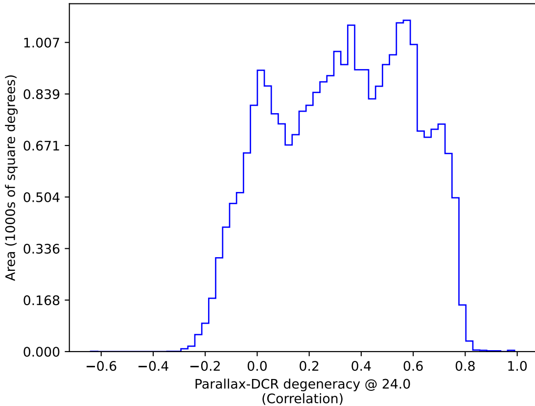
ddf_acor_sf15_ls30_lsr10_v3.4_10yrs : Parallax-DCR degeneracy @ 24.0
