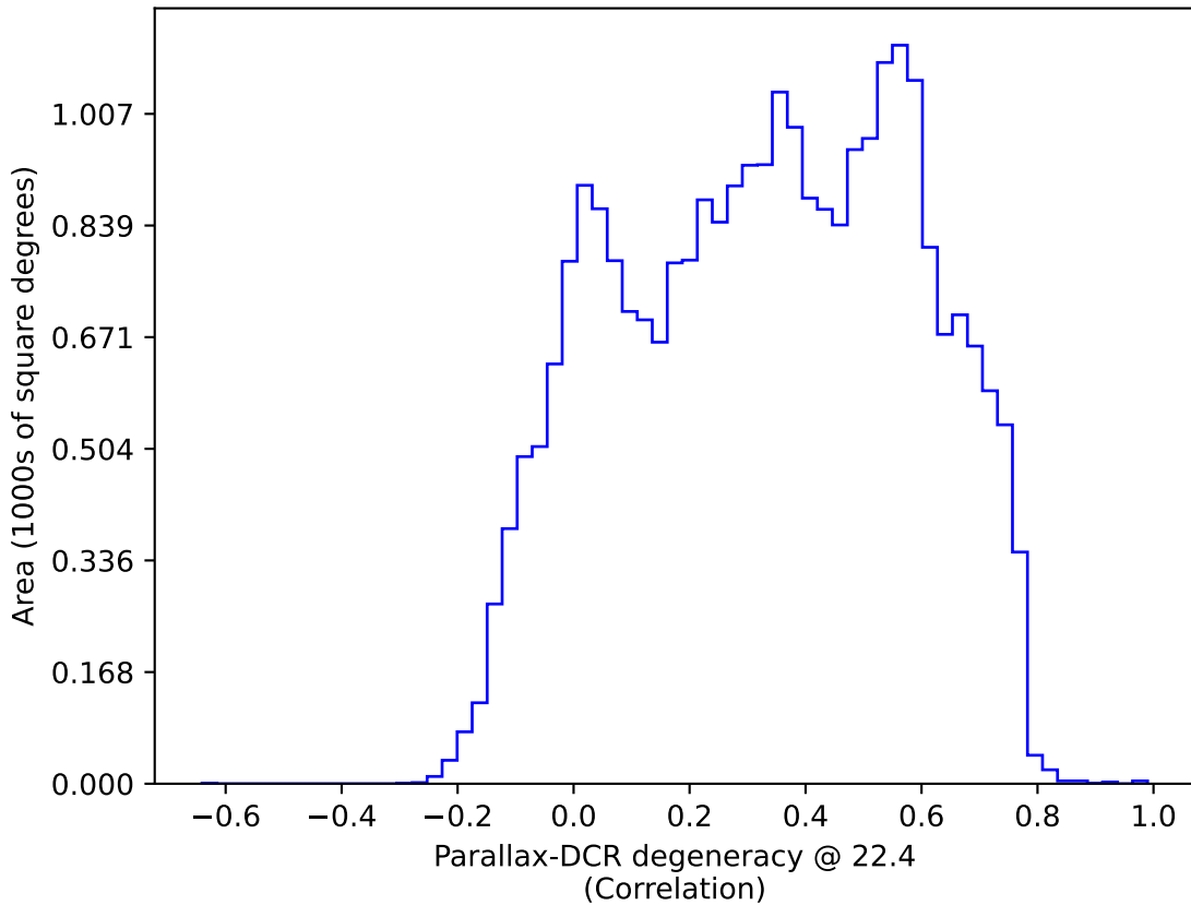
ddf_acor_sf15_lsf30_lsr10_v3.4_10yrs : Parallax-DCR degeneracy @ 22.4
