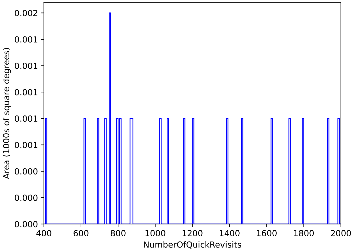
ddf_acor_sf15_lsf30_lsr10_v3.4_10yrs : NumberOfQuickRevisits
