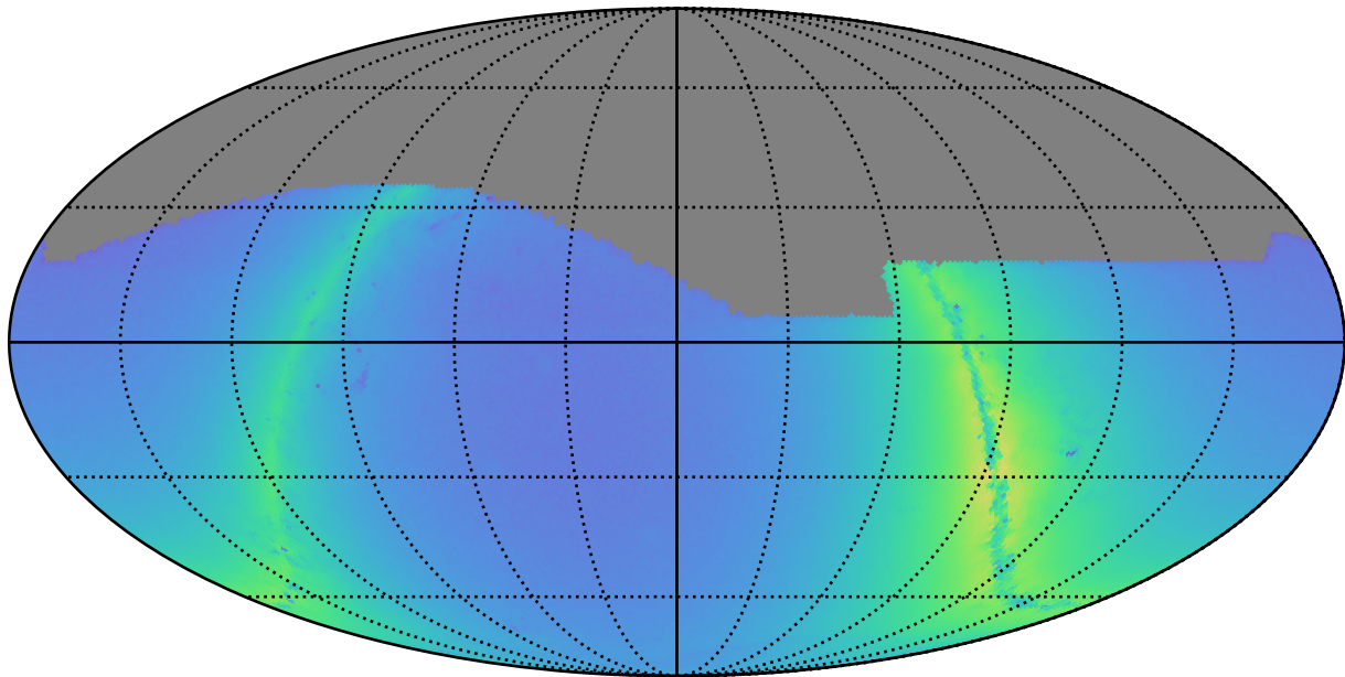
ddf_acor_sf15_lsf30_lsr10_v3.4_10yrs r: Nstars_no_crowding
