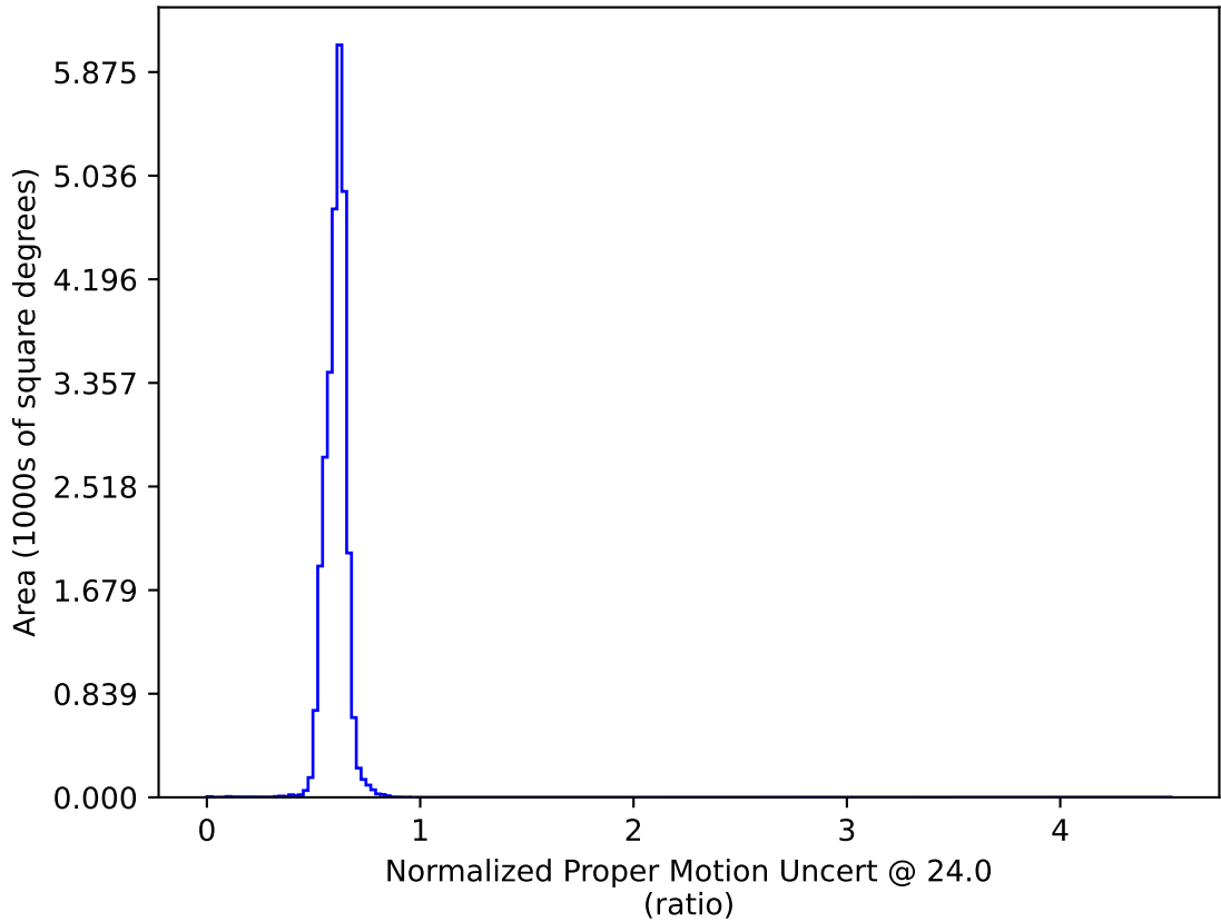
ddf_acor_sf15_lsf30_lsr10_v3.4_10yrs : Normalized Proper Motion Uncert @ 24.0
