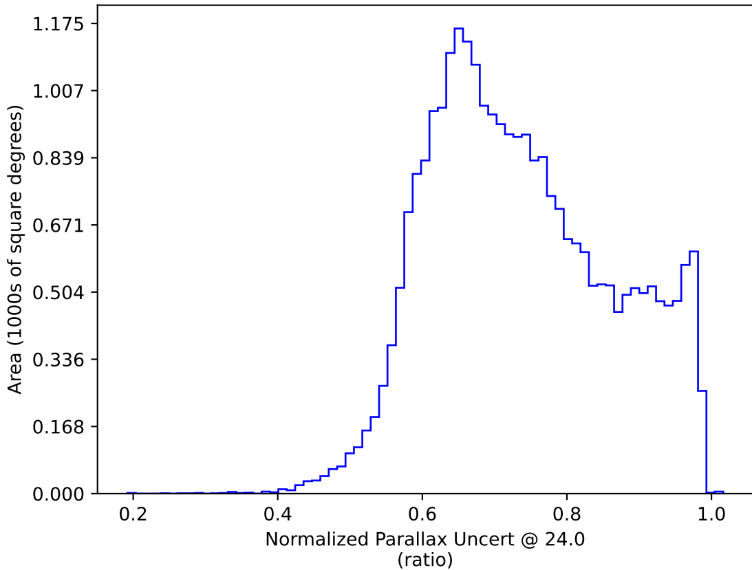
ddf_acor_sf15_lsf30_lsr10_v3.4_10yrs : Normalized Parallax Uncert @ 24.0
