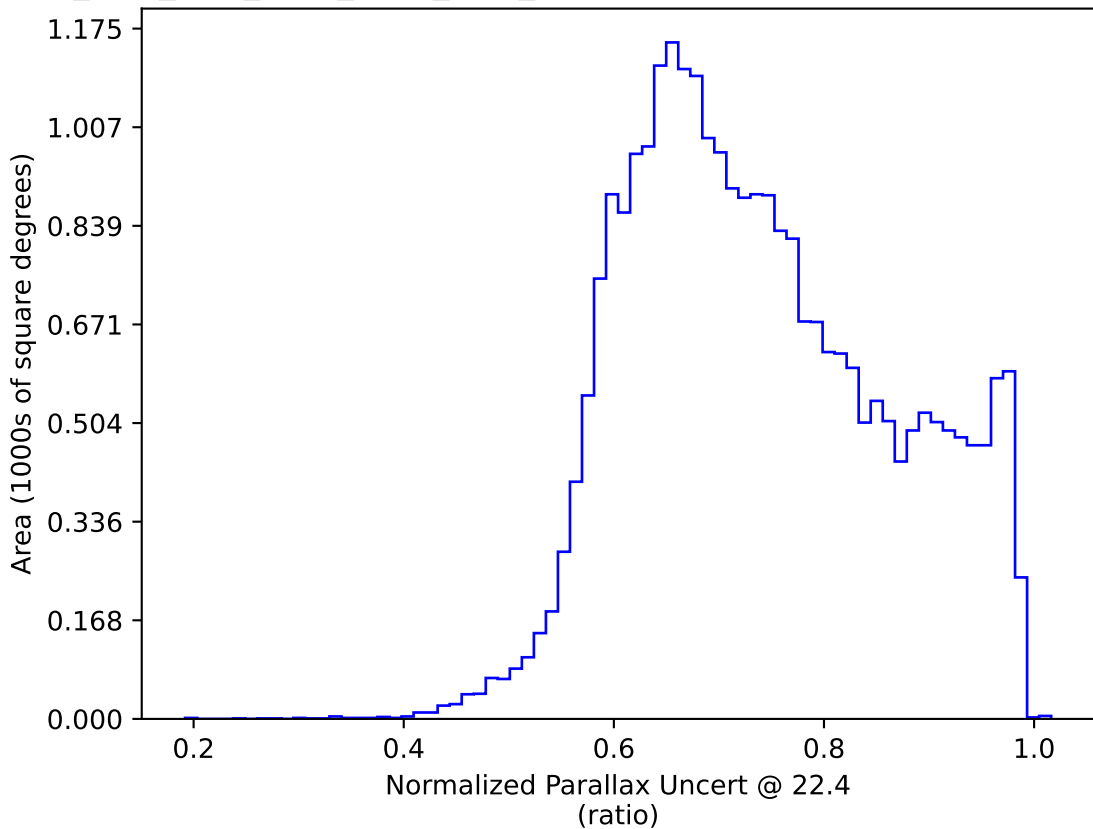
ddf_acor_sf15_lsf30_lsr10_v3.4_10yrs : Normalized Parallax Uncert @ 22.4
