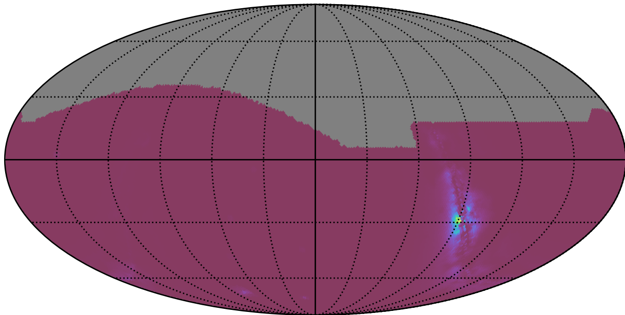
ddf_acor_sf15_lsf30_lsr10_v3.4_10yrs : NlcPoints
