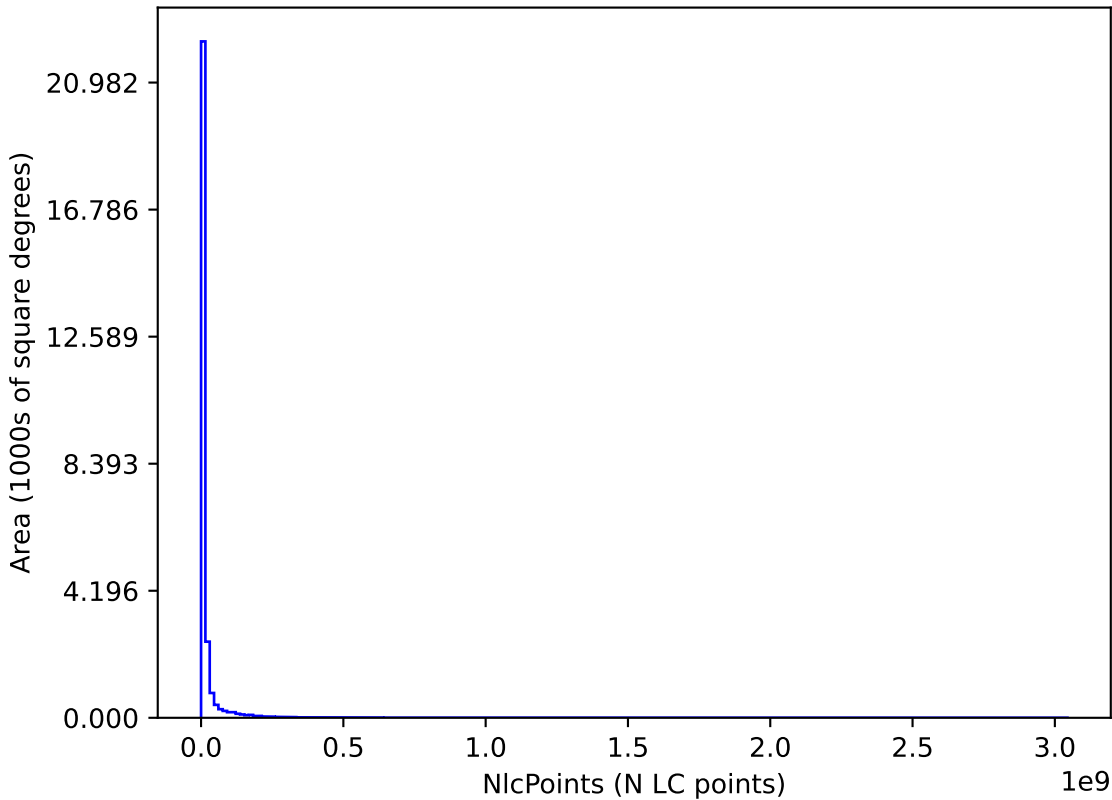
ddf_acor_sf15_lsf30_lsr10_v3.4_10yrs : NlcPoints
