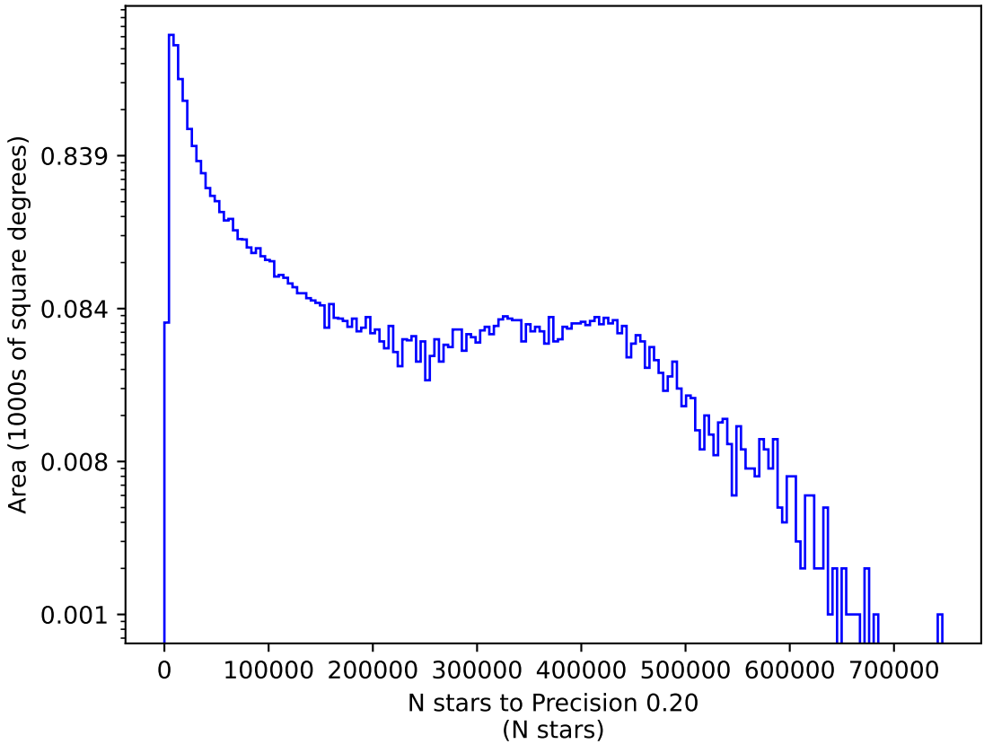
ddf_acor_sf15_lsf30_lsr10_v3.4_10yrs r: N stars to Precision 0.20
