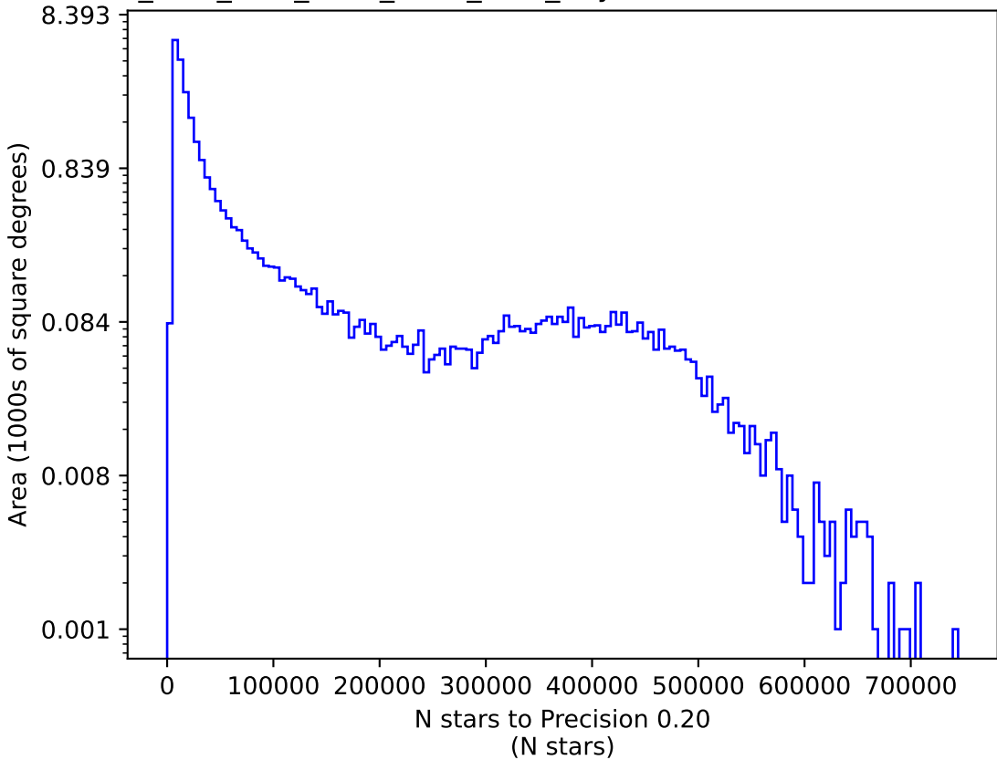
ddf_acor_sf15_lsf30_lsr10_v3.4_10yrs i: N stars to Precision 0.20
