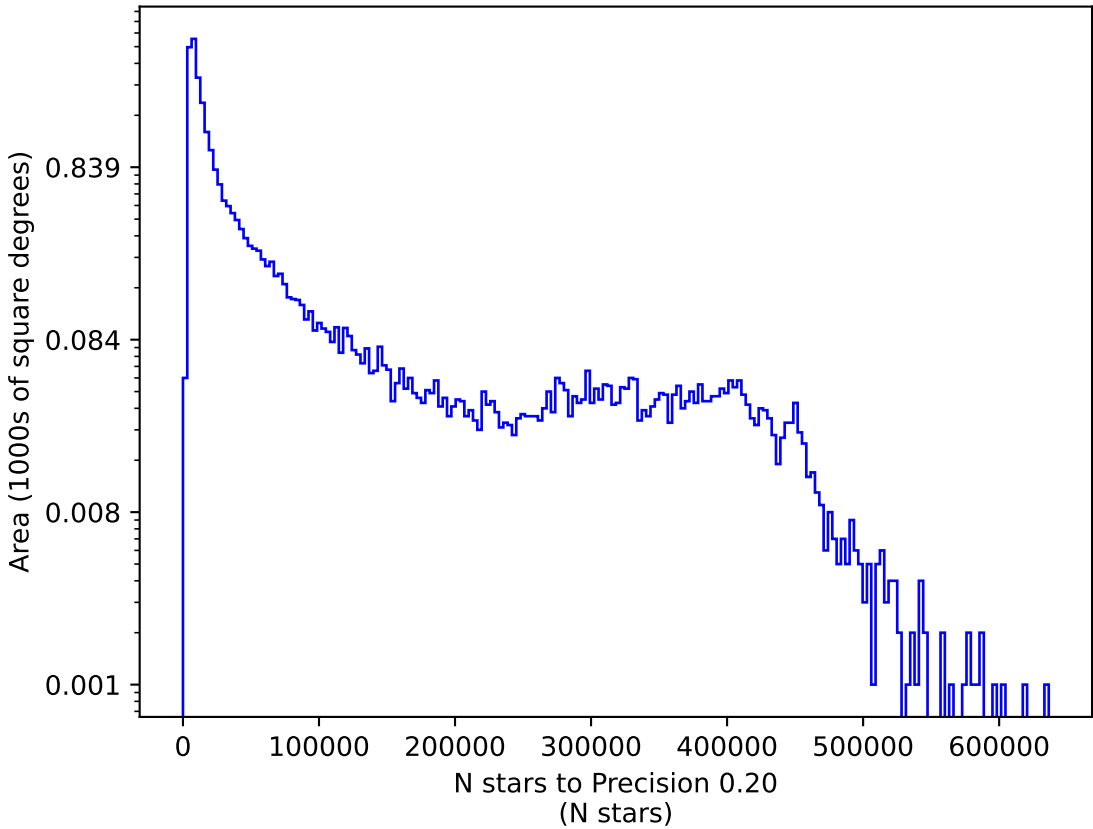
ddf_acor_sf15_lsf30_lsr10_v3.4_10yrs g: N stars to Precision 0.20
