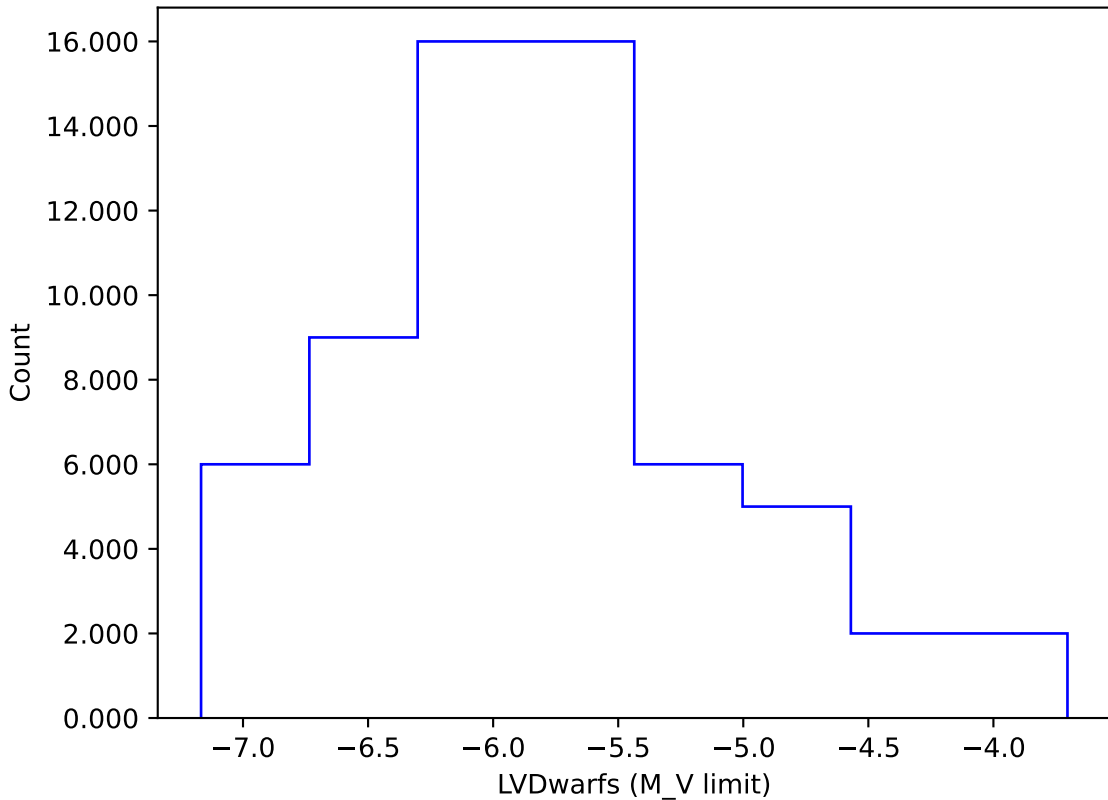
ddf_acor_sf15_lsf30_lsr10_v3.4_10yrs gi: LVDwarfs
