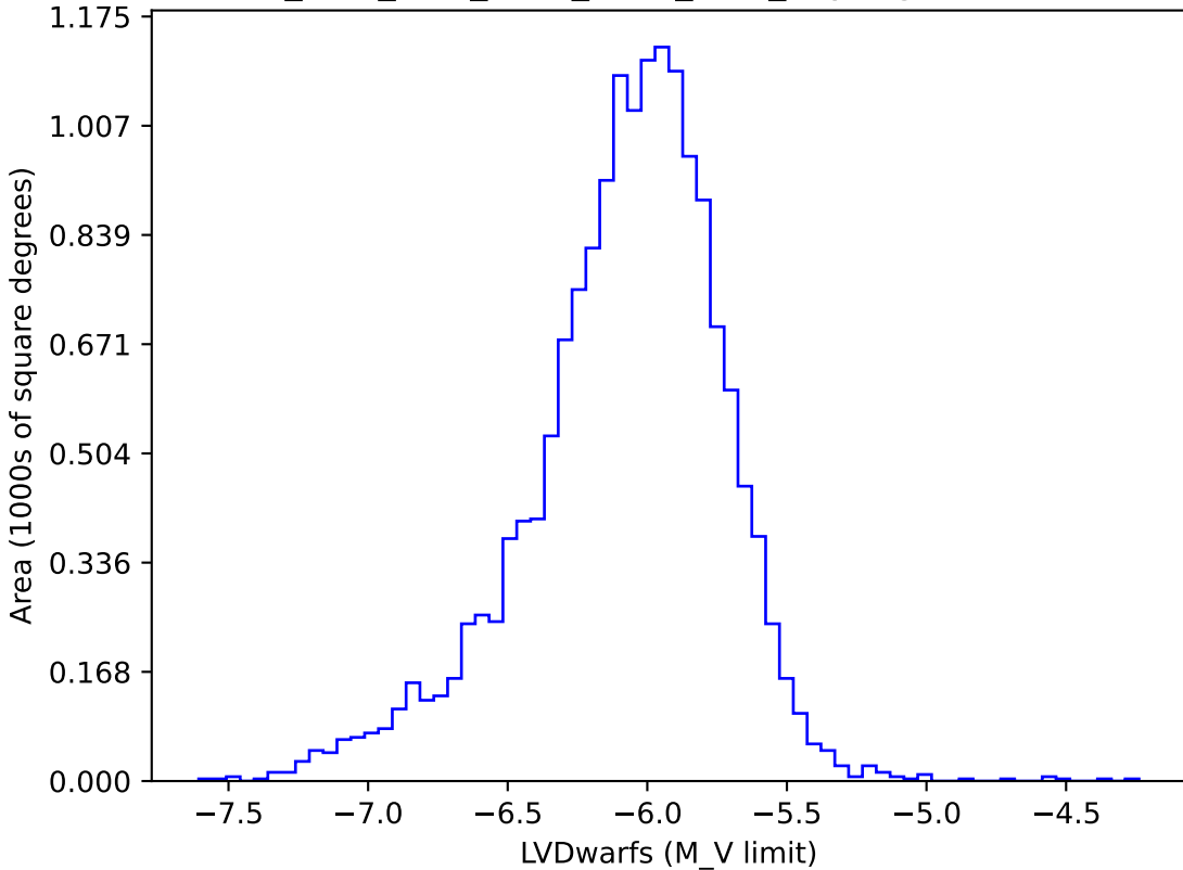
ddf_acor_sf15_lsf30_lsr10_v3.4_10yrs gi: LVDwarfs
