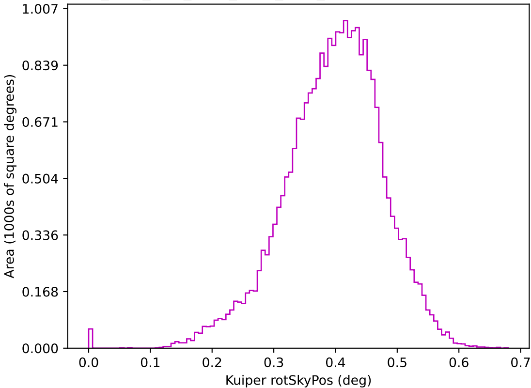
ddf_acor_sf15_lsf30_lsr10_v3.4_10yrs z: Kuiper rotSkyPos
