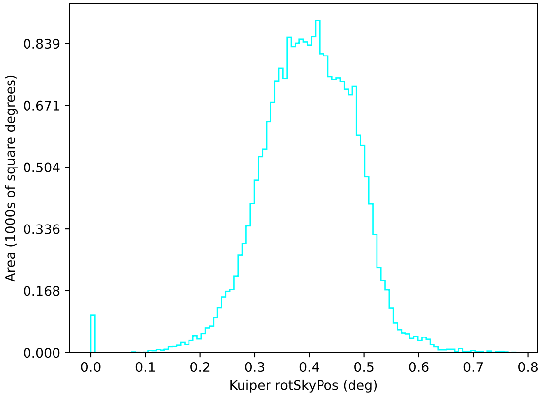
ddf_acor_sf15_lsf30_lsr10_v3.4_10yrs u: Kuiper rotSkyPos
