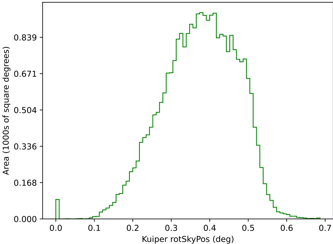
ddf_acor_sf15_lsf30_lsr10_v3.4_10yrs g: Kuiper rotSkyPos
