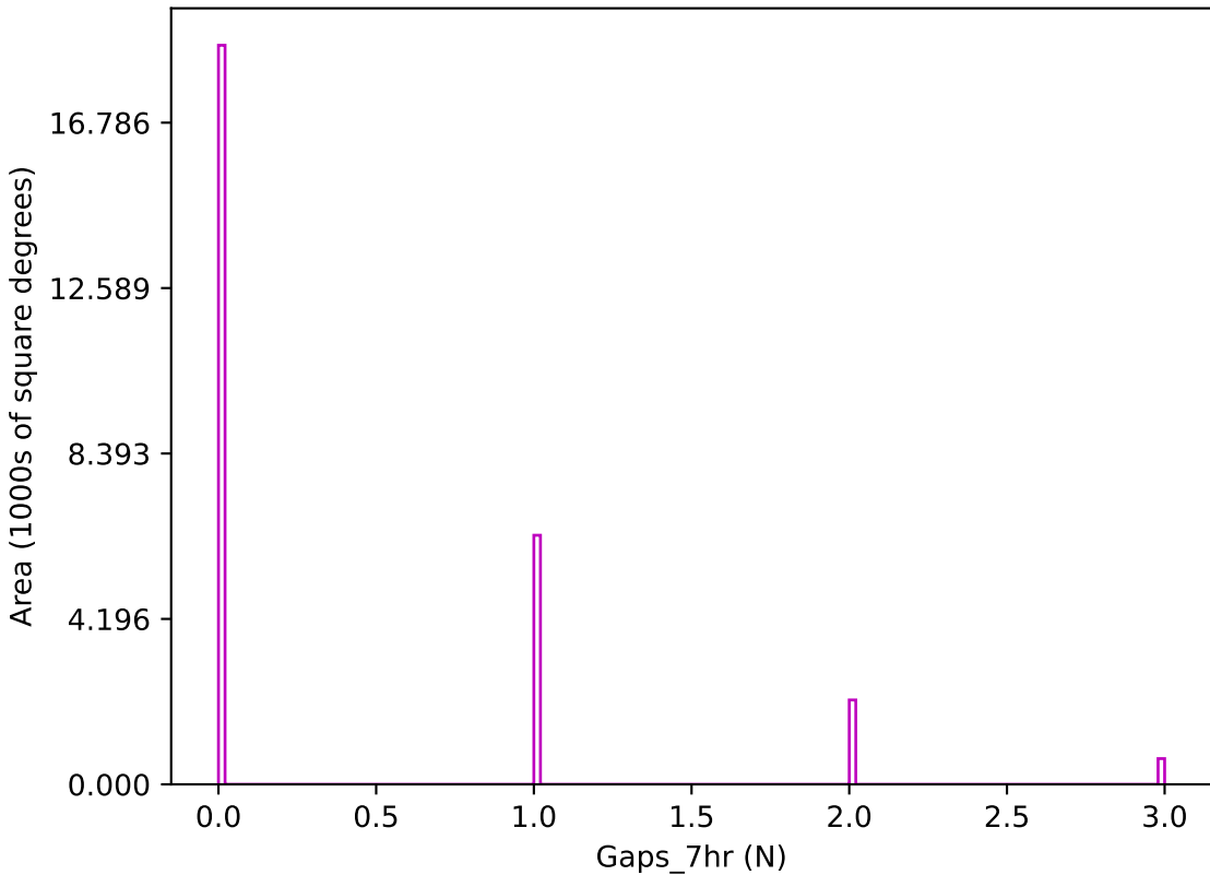
ddf_acor_sf15_ls30_lsr10_v3.4_10yrs z band: Gaps_7hr
