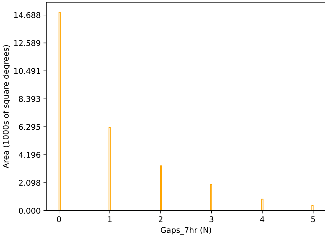
ddf_acor_sf15_lsf30_lsr10_v3.4_10yrs r band: Gaps_7hr
